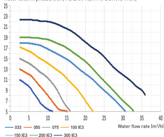
Water column pressure (m) KS Evo / KSX Pro Q (m 3 /h)-H (m)
